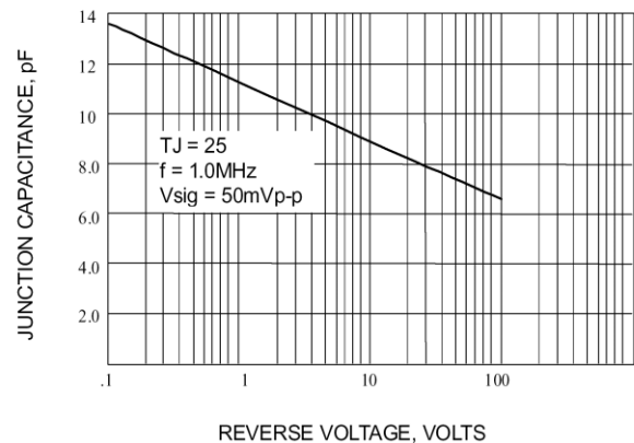
Fig. 6-TYPICAL JUNCTION CAPACITANCE
